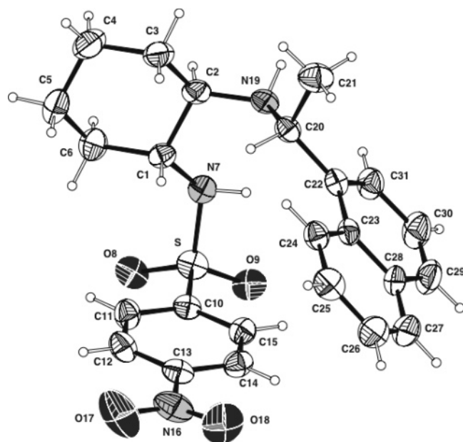
Figure 1. X-ray crystal structure of (1R,2R,1'R)-7d.
