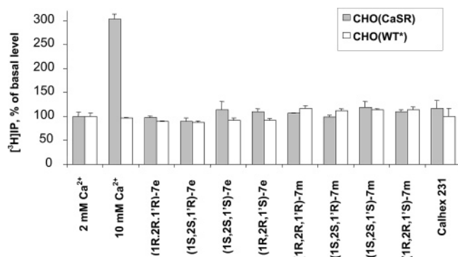
Figure 4. Basal activity of compound Calhex 231 compared to the four different isomers of 7e and 7m . Compounds at 10 \mu M were applied to CHO (CaSR) or CHO (WT*) cells in the presence of a basal level of extracellular \text{Ca}^{2+} (2 mM). In both cell types, compounds, including Calhex 231, had limited effects on IP production. Data (mean \pm SEM) are expressed as the percentage of the basal response. Maximal response on IP accumulation was evaluated at 10 mM extracellular \text{Ca}^{2+} .
