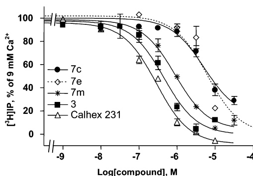
Figure 2. Calcilytic potency of selected compounds 7 compared to compound 3 : concentration response curves for inhibition of calcium induced IP accumulation in CHO (CaSR) cells. Data (mean \pm SEM) are expressed as the percentage of 9 mM extracellular \text{Ca}^{2+} IP response over the basal level at 2 mM extracellular \text{Ca}^{2+} : 7c , \text{IC}_{50} = 8 \pm 2 \mu\text{M} ; 7e , \text{IC}_{50} = 5.4 \pm 0.5 \mu\text{M} ; 7m , \text{IC}_{50} = 0.9 \pm 0.2 \mu\text{M} ; 3 , \text{IC}_{50} = 0.46 \pm 0.05 \mu\text{M} ; (1 S ,2 S ,1' R )- 7n (Calhex 231), \text{IC}_{50} = 0.33 \pm 0.02 \mu\text{M} .
