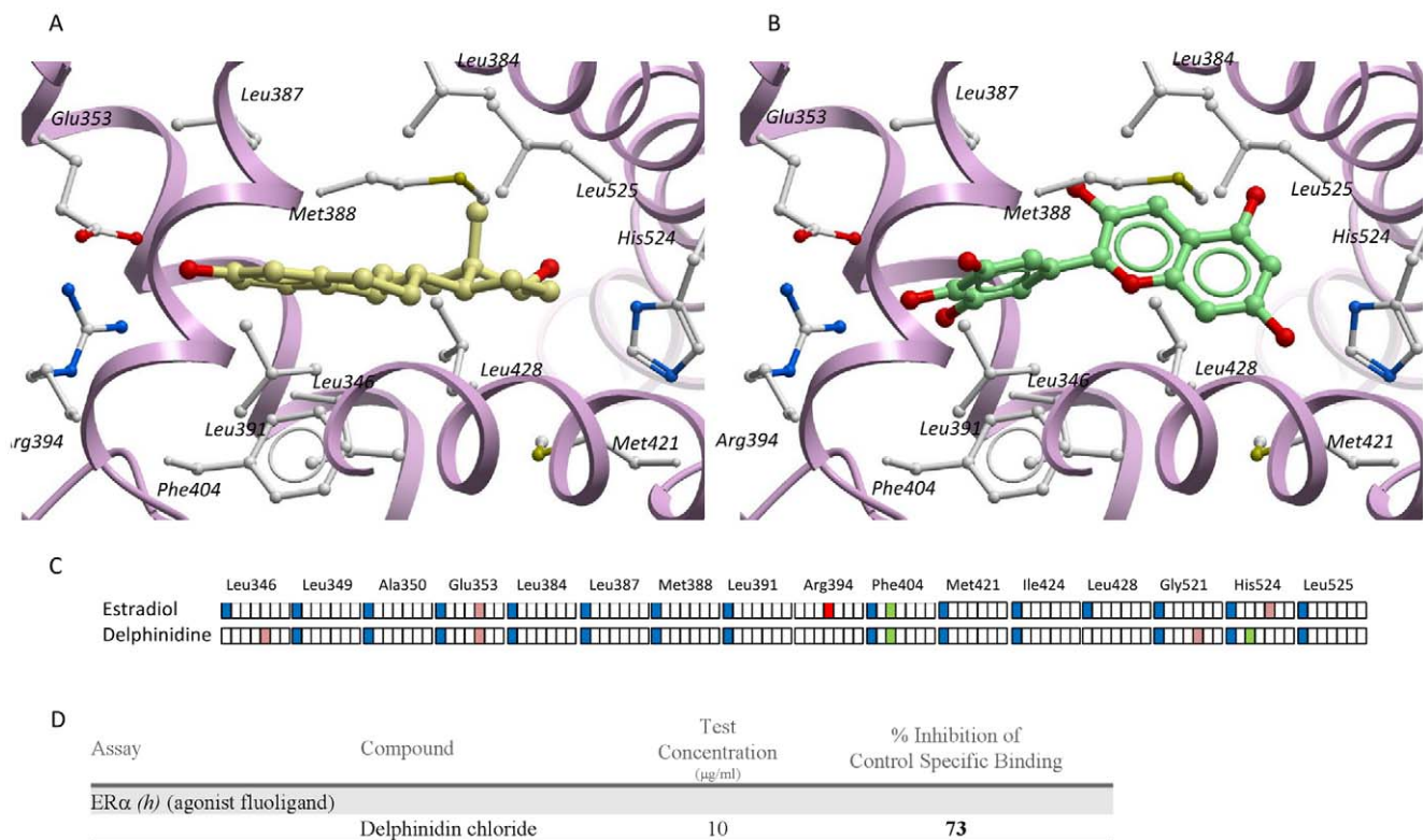
Figure 4. Binding assay and docking show direct interaction between delphinidin and ER \alpha activator site. Binding mode of 17- \beta estradiol (E 2 ) (panel A, X-ray structure) and delphinidin (panel B, docking model) to the ligand-binding domain of the ER \alpha (1a52 PDB entry). The receptor backbone is displayed by solid ribbons. Ligand-contacting side chains are displayed by white ball and sticks. Carbon atoms of receptor-bound E 2 and delphinidin are in yellow and green, respectively. In panel C, the ligand-receptor interactions for both compounds are encoded by an interaction fingerprint converting into a 7 bit string the interaction of the ligand with each residue of the binding site using the following color-coding: blue, apolar contact; green: aromatic interaction; red: hydrogen-bond. Eventually, D represents results of a binding assay of delphinidin on ER \alpha . E 2 was used as control agonist for ER \alpha and delphinidin was used at concentration exerting endothelial effects shown before ( 10^{-2} g/L). doi:10.1371/journal.pone.0008554.g004
